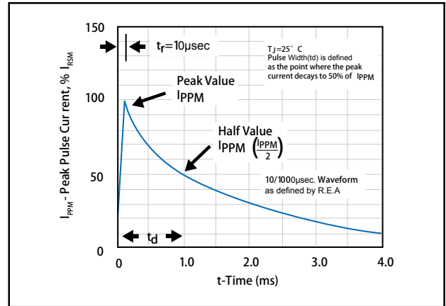
Figure 4 - Pulse Waveform
