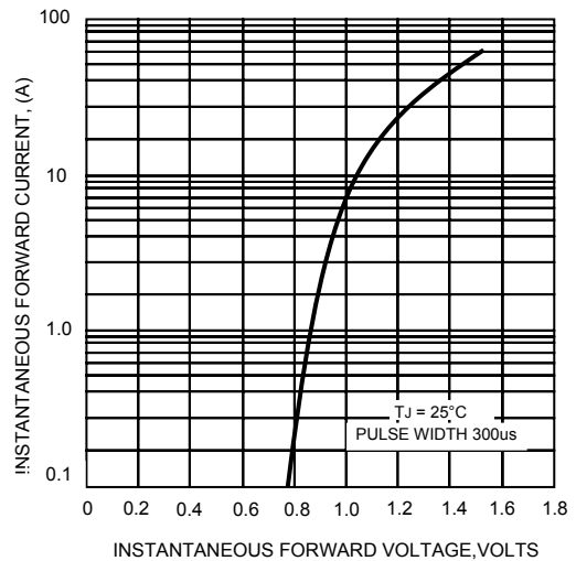
FIG.4-TYPICAL FORWARD CHARACTERISTICS
