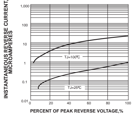
FIG. 4-TYPICAL REVERSE CHARACTERISTICS
