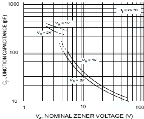
Fig. 5 Junction Capacitance vs Nominal Zener Voltage
