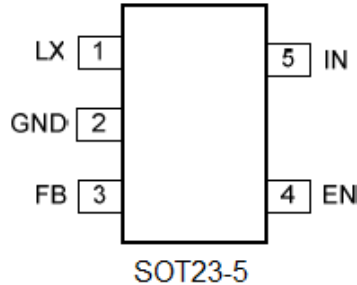
Figure 2 Pin Configuration of TD8210(Top View)
