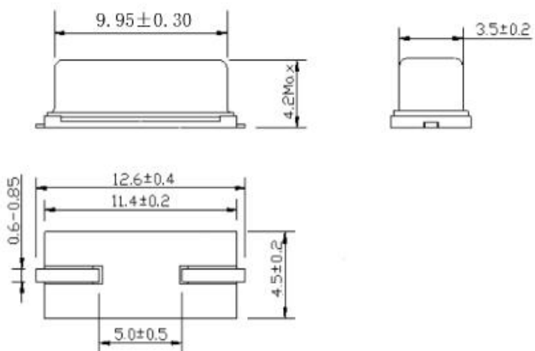
Dimensions(mm)
