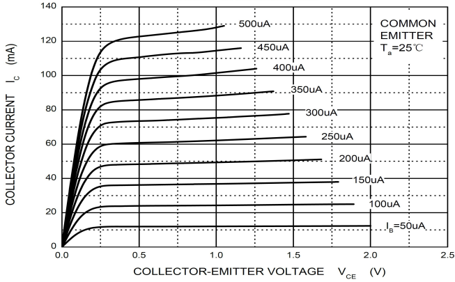
Static Characteristic
