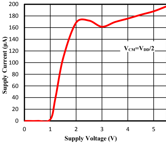
Figure 1. Supply Current vs. Supply Voltage
