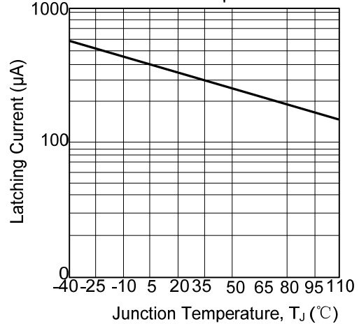
Typical Latching Current vs. Junction Temperature
