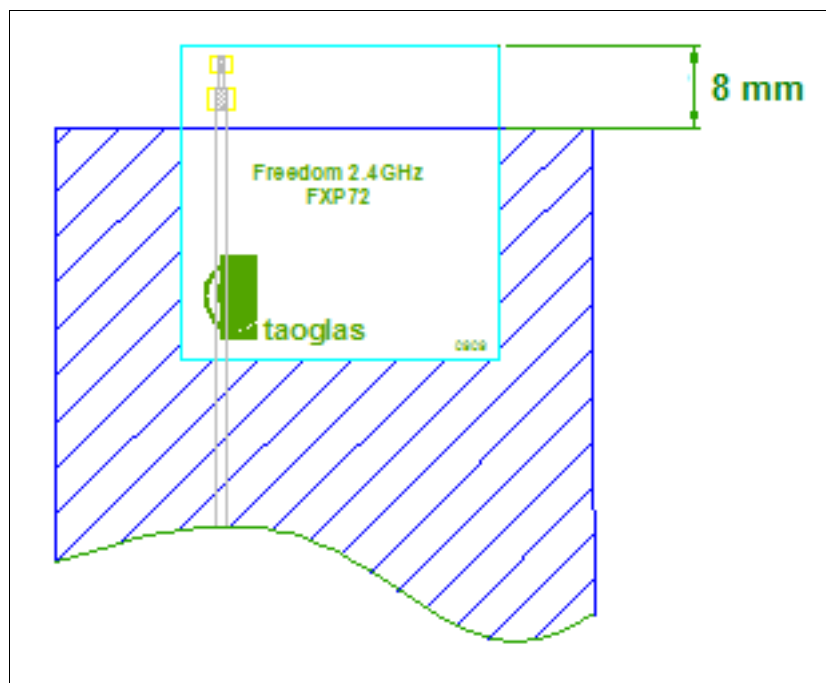
Figure 12. Mounting Guidelines.
