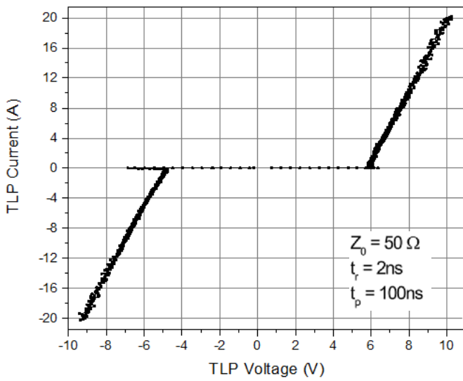
Fig5.TLP Measurement
