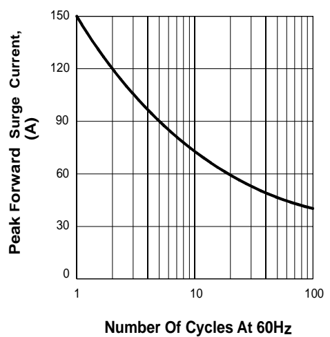
FIG.4 PEAK FORWARD SURGE CURRENT
