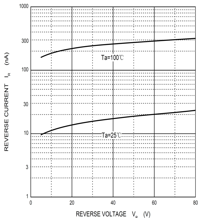
Reverse Characteristics
