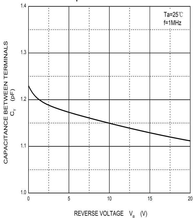
Capacitance Characteristics
