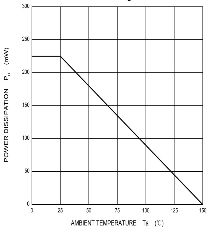
Power Derating Curve
