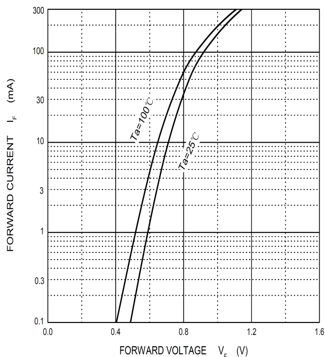
Forward Characteristics
