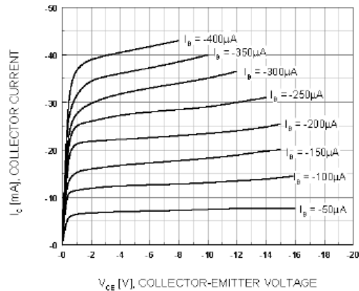
Figure 1. Static Characteristic
