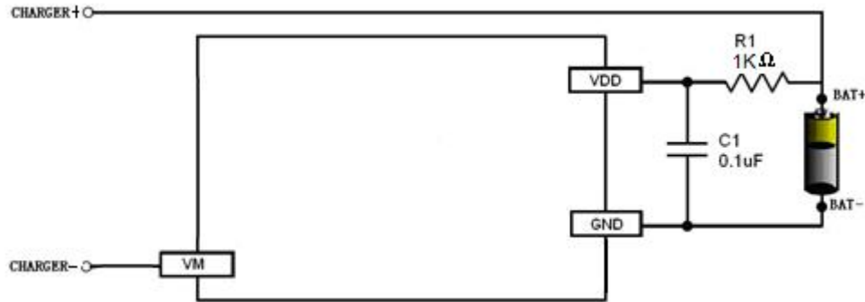
Fig 6 XB3306A in a Typical Battery Protection Circuit
