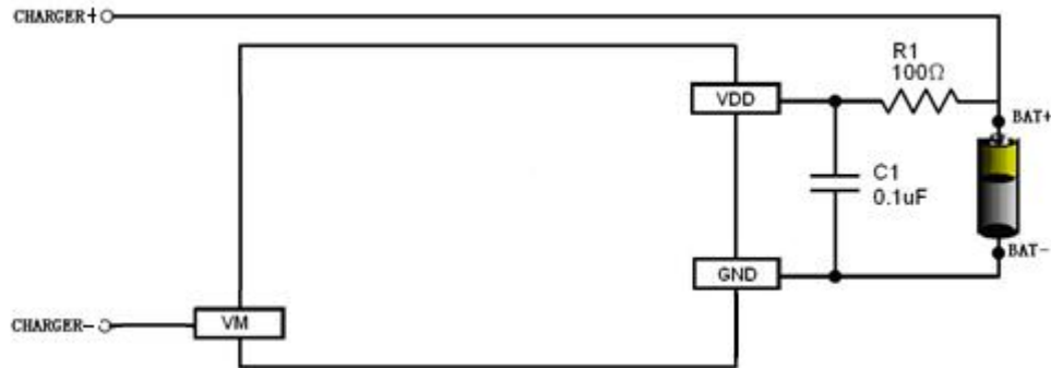
Fig 6 XB3303G in a Typical Battery Protection Circuit
